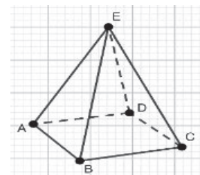
Pirâmide rectangular
