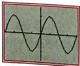
y = \sin x
