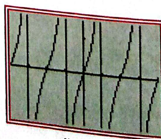
y = \tan x
